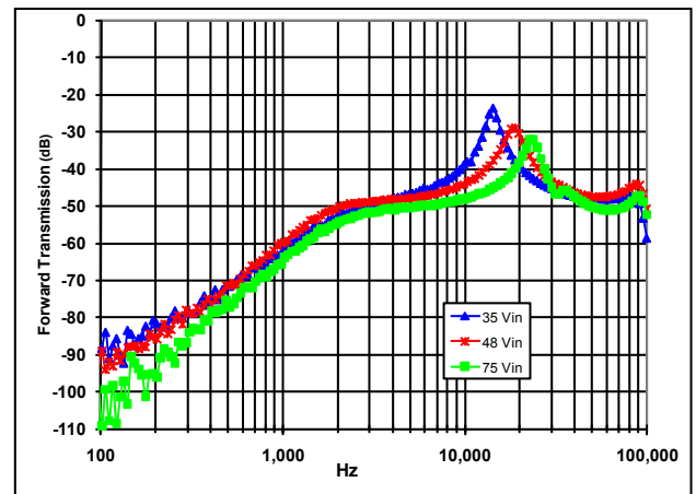
Figure 22: Magnitude of incremental forward transmission ( FT = v_{out}/v_{in} ) for minimum, nominal, and maximum input voltage at full rated power.
