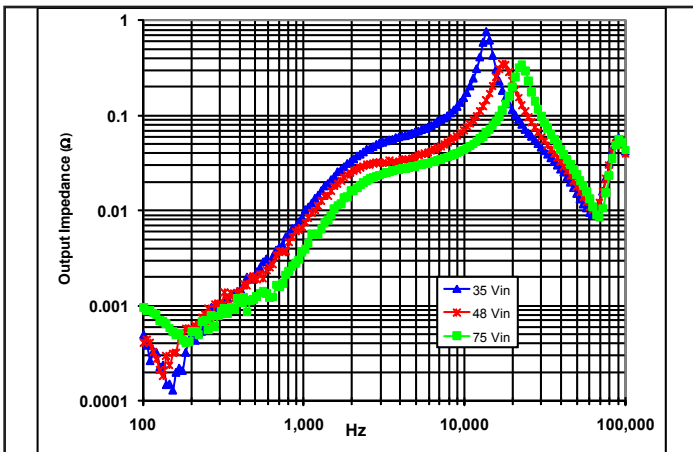
Figure 21: Magnitude of incremental output impedance ( Z_{out} = v_{out}/i_{out} ) for minimum, nominal, and maximum input voltage at full rated power.
