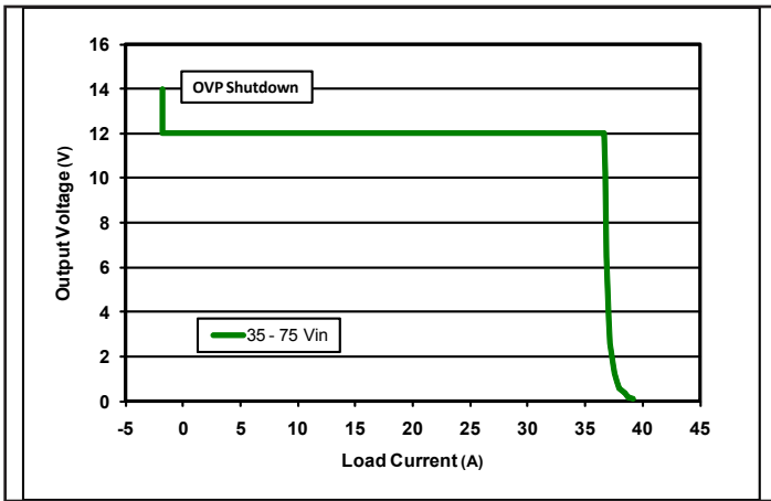
Figure 19: Output voltage vs. load current showing typical current limit curves and OVP shutdown point.
